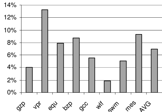
Figure 4: Performance improvement achieved by bypassing trivial instructions over a conventional processor.
