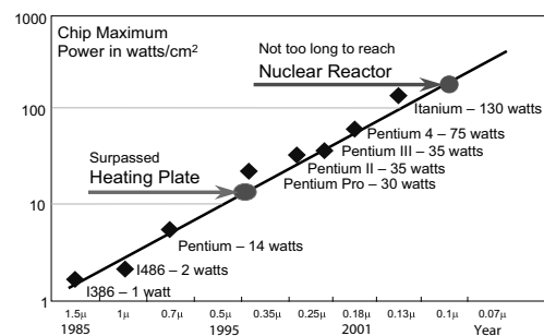
Figure 1. Moore's Law for Power Consumption.
